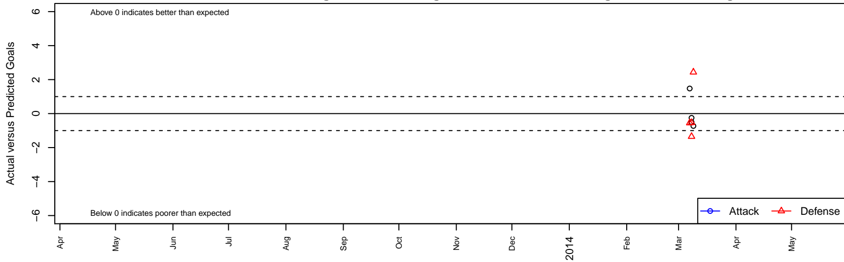
Heat FC 97 BJ B96 Dots are actual minus expected GF (blue circles) and GA (red triangles). Blue line is smoothed change in attack strength. Red is smoothed change in defense strength.
